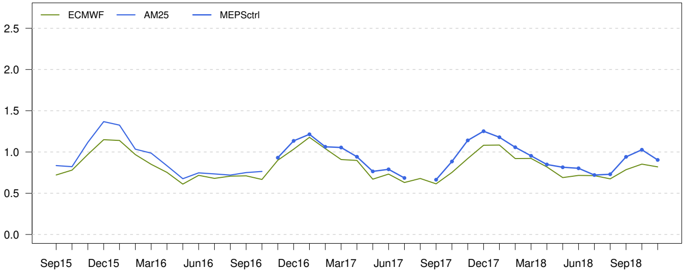
Mean Absolute Error 119 Norwegian stations
